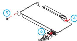
2-9 显卡安装
