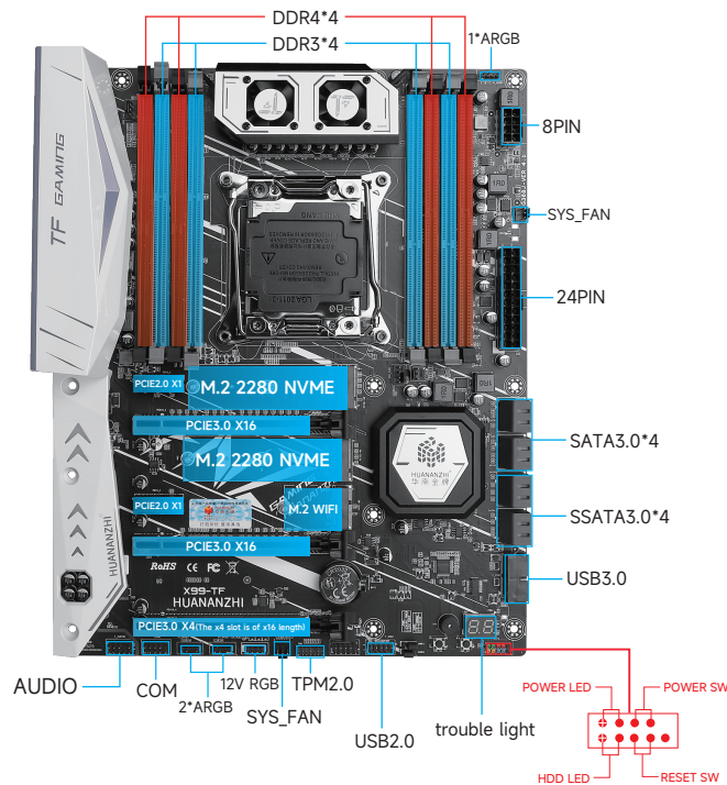
1-1 X99-TF Motherboard Illustration
