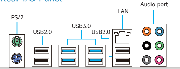
1-2 Overall Rear I/O Panel Display
